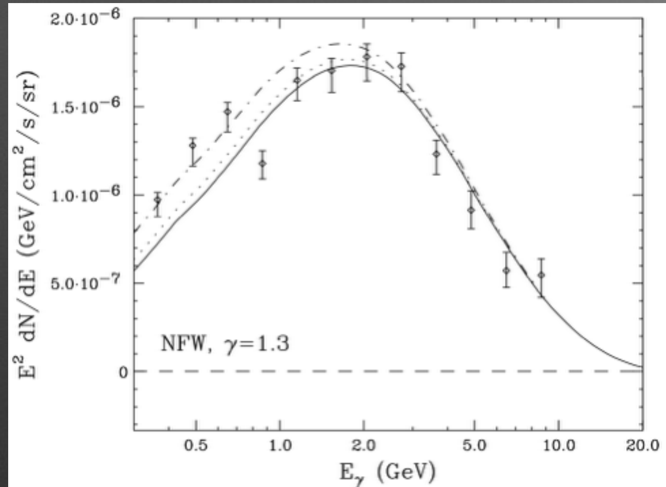
Galactic Center
