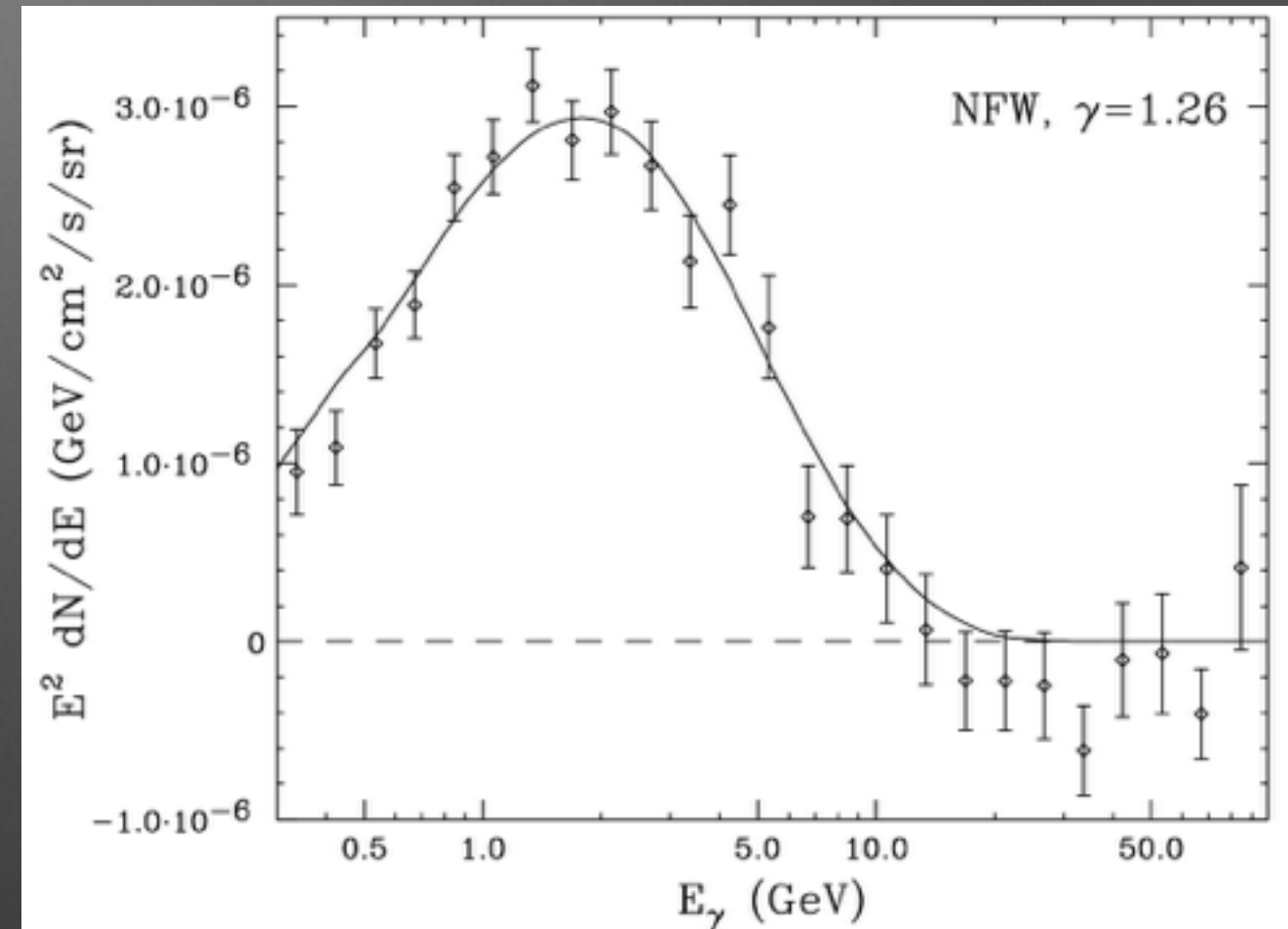
Inner Galaxy
